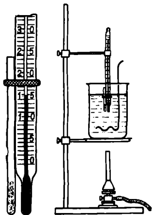
Fig. 18. Apparatus for determining melting point
