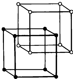
Fig. 173. Diagram of the structure of CsCl
