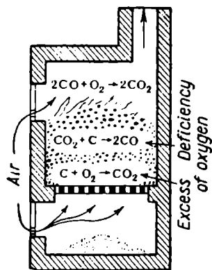
Fig. 135. Formation and combustion of CO in a furnace
