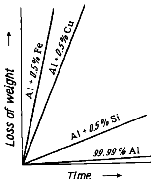
Fig. 151. Effect of admixtures on the rate of solution of Al in HCl
