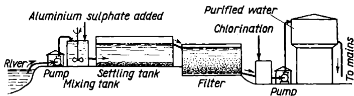
Fig. 73. Diagram of the purification of river water
