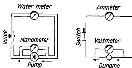
Fig. 93. Analogy between a water and an electrical system
