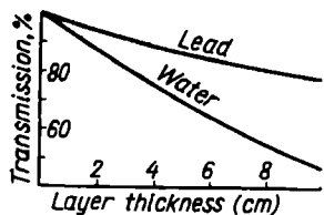
Fig. 230. Transparency to fast neutrons
