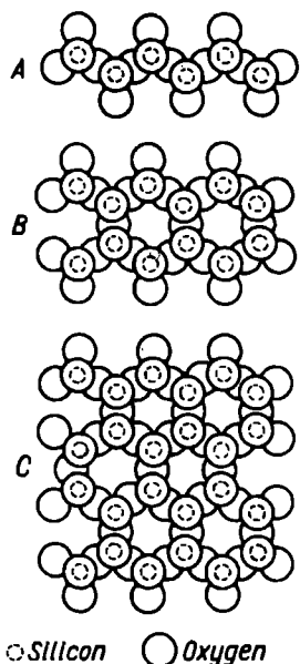
Fig. 143. Group silicate structures
