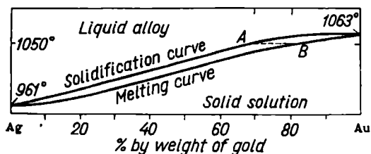
Fig. 164. Freezing-point diagram for the system Ag—Au
