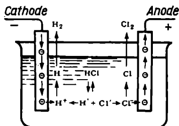
Fig. 94. Diagram of electrolysis
