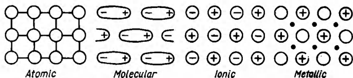
Fig. 54. Basic structures of solids
