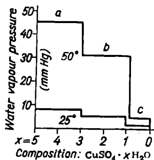
Fig. 157. Crystal hydrates of \text{CuSO}_4
