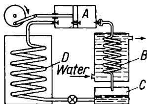
Fig. 114. Diagram of a refrigerator
