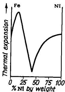
Fig. 156. Thermal expansion of Fe—Ni alloys
