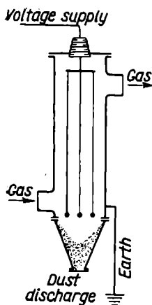
Fig. 148. Electrostatic precipitator
