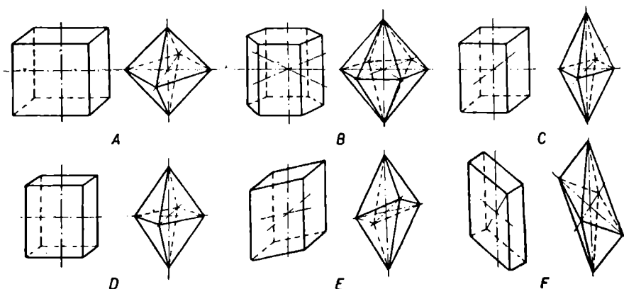
Fig. 167. Prismatic and pyramidal crystals
