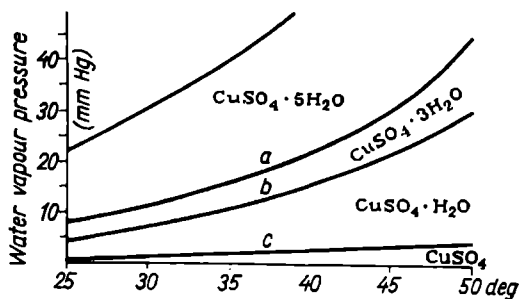
Fig. 158. Stability regions of the hydrated forms of \text{CuSO}_4
