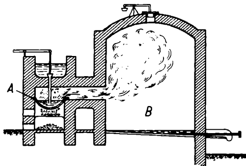
Fig. 102. Sulphur-distillation kiln
