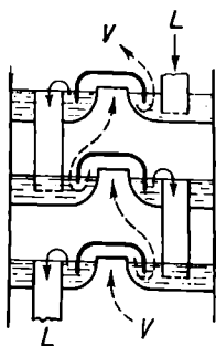
Fig. 13. Diagram of operation of the plates in a separating column
