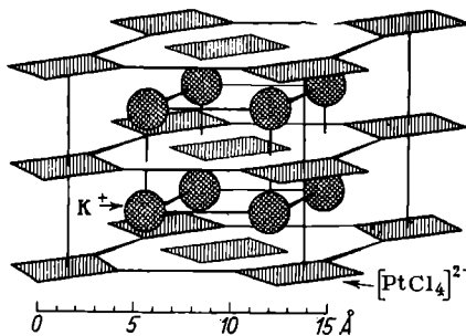
Fig. 200. Crystal structure of K_2[PtCl_4]
