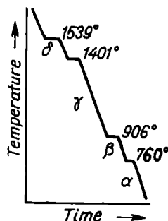
Fig. 154. Cooling curve of iron
