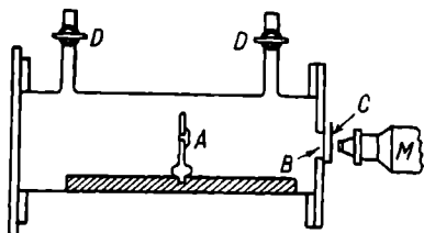
Fig. 225. Diagram of Rutherford's apparatus
