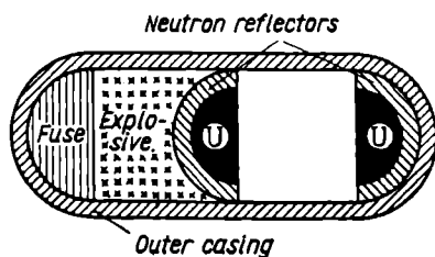
Fig. 234. Diagram of the simplest atomic bomb
