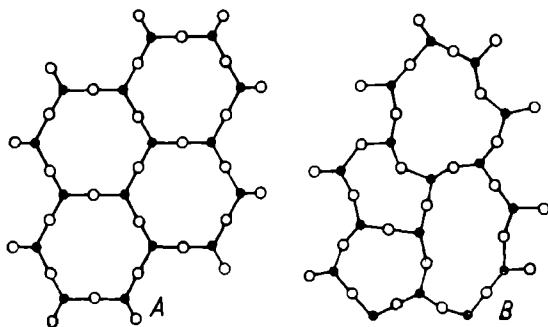
Fig. 145. Arrangement of atoms in \text{Al}_2\text{O}_3 in the crystalline and vitreous states
