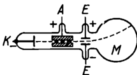
Fig. 24. Diagram of apparatus for investigating cathode rays
