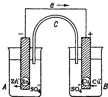
Fig. 90. A galvanic cell
