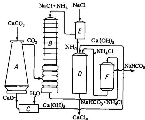
Fig. 192. Production of soda by the Solvay process
