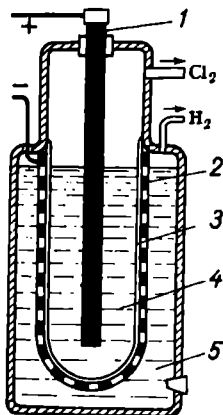
Fig. 96. Electrolytic cell for producing chlorine:
