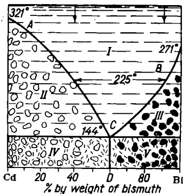
Fig. 160. Freezing-point diagram for the system Cd—Bi
