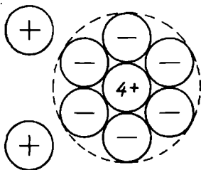
Fig. 116. Structure of \text{Na}_2\text{SiF}_6
