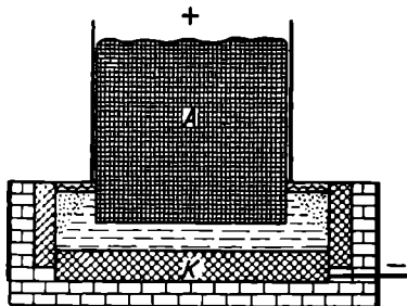
Fig. 150. Diagram of electric furnace for the production of aluminium
