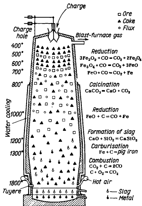
Fig. 202. Diagram of the blast-furnace process
