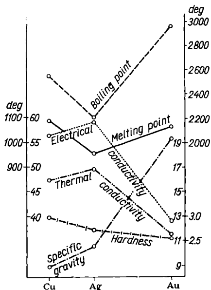
Fig. 196. Properties of Cu, Ag and Au
