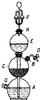
Fig. 58. Apparatus for producing gases
