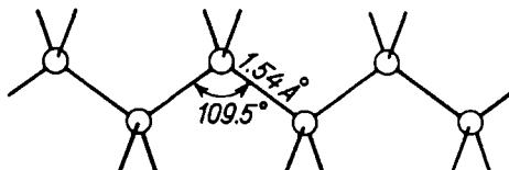
Fig. 140. Structure of a carbon chain
