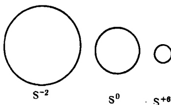
Fig. 57. Influence of valency state on size of atom
