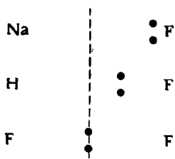
Fig. 41. Diagram of the types of valency bonds
