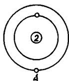
Fig. 35. Possible models of the helium atom
