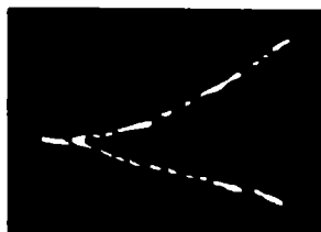
Fig. 221. Tracks of an electron-positron pair
