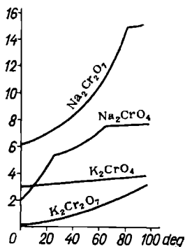
Fig. 109. Solubility of chromates and dichromates (moles/litre of \text{H}_2\text{O} )
