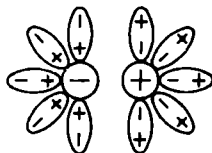
Fig. 85. Orientation of dipoles about an ionic molecule
