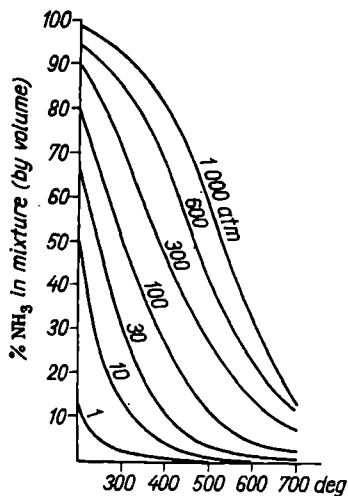
Fig. 110. Equilibrium of ammonia synthesis from its elements
