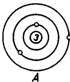
Fig. 36. Possible models of the lithium atom
