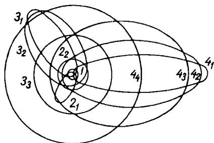
Fig. 66. Possible electronic orbits in the hydrogen atom after Sommerfeld
