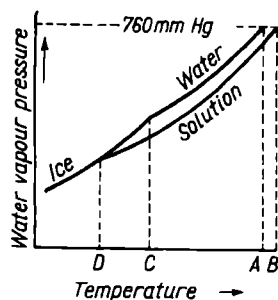
Fig. 83. Vapour pressure of water and of a solution
