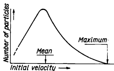
Fig. 214. Distribution of velocities of \beta -particles
