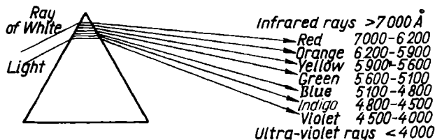
Fig. 12. Splitting up of a sun beam by a prism
