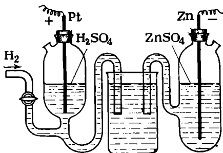
Fig. 92. Determination of electrode potential
