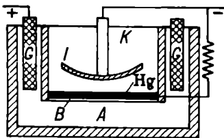
Fig. 187. Installation for electrolysis by the mercury method
