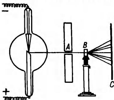
Fig. 52. Arrangement for investigating the internal structure of crystals
