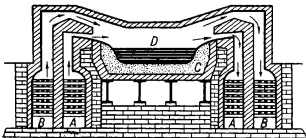
Fig. 204. Open-hearth furnace
