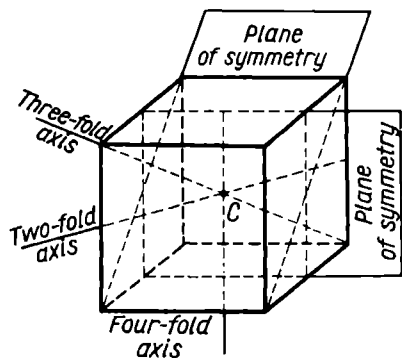
Fig. 168. Elements of symmetry of a cube
