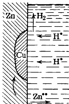
Fig. 91. A galvanic couple
