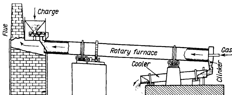
Fig. 181. Cement kiln
