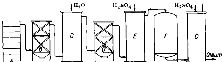
Fig. 106. Diagram of contact plant for manufacture of sulphuric acid
