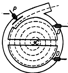
Fig. 227. Diagram of a cyclotron
