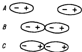
Fig. 47. Diagram of interaction between polar molecules
