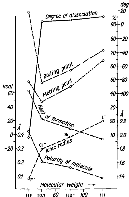
Fig. 100. Properties of the hydrogen halides
