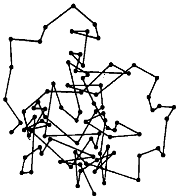
Fig. 20. Path of a gas particle
