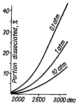
Fig. 72. Equilibrium of the thermal dissociation of water
