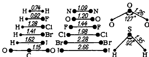
Fig. 44. Arrangement of atomic nuclei in some of the simplest molecules
