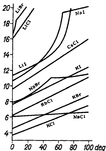
Fig. 188. Solubility of halides (moles/litre of \text{H}_2\text{O} )
