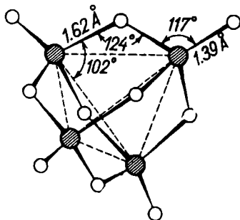
Fig. 126 Spatial structure of \text{P}_4\text{O}_{10}
