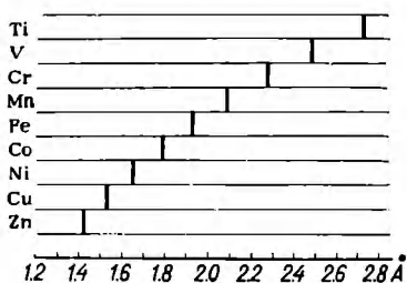
Fig. 33. X-ray wavelengths for the elements from Ti to Zn
