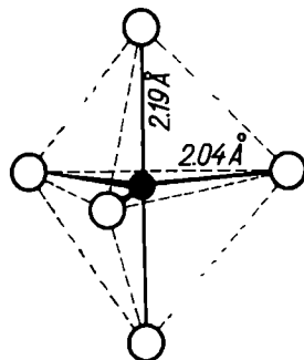
Fig. 128. Structure of \text{PCl}_5 molecule
