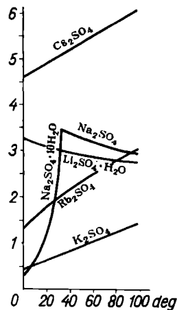
Fig. 193. Solubility of sulphates (moles/litre of \text{H}_2\text{O} )
