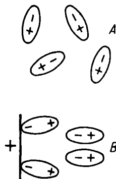
Fig. 46. Polarisation of polar molecules
