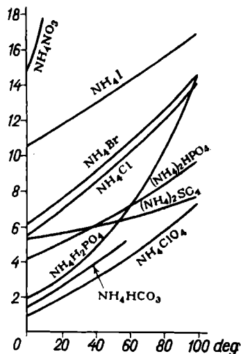
Fig. 115. Solubility of ammonium salts (moles/litre of \text{H}_2\text{O} )
