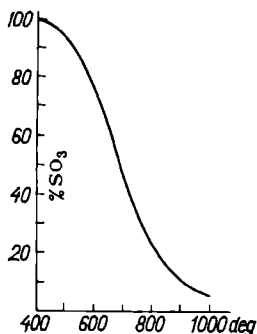
Fig. 104. Equilibrium of thermal dissociation of \text{SO}_3
