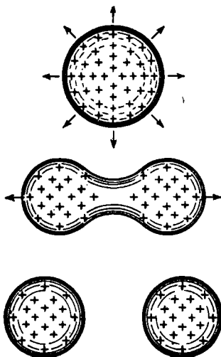
Fig. 231. Division of a charged drop
