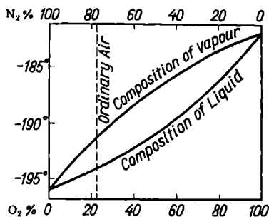
Fig. 11. Boiling point vs. composition of liquid air
