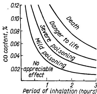
Fig. 134. Effect of carbon monoxide on a human being
