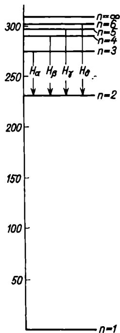
Fig. 65. Energy levels of the hydrogen atom (kcal/gram-atom)
