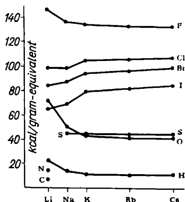
Fig. 186. Heats of formation of the compounds of the alkali metals
