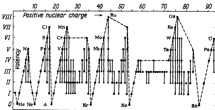
Fig. 210. Valencies of the chemical elements'
