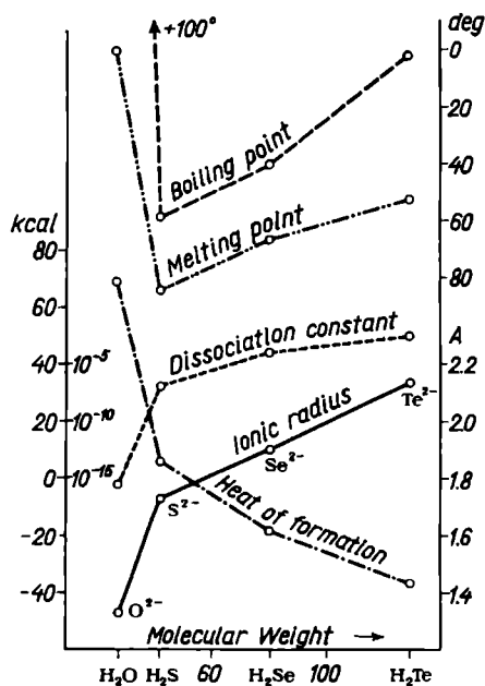
Fig. 108. Properties of hydrogen compounds of group VI elements
