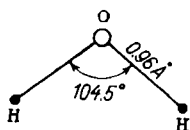
Fig. 74. Arrangement of atomic nuclei in the water molecule
