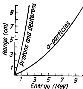
Fig. 228. Range in air vs. energy of particles
