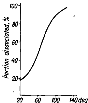
Fig. 118. Equilibrium of the system \text{N}_2\text{O}_4 \rightleftharpoons 2\text{NO}_2
