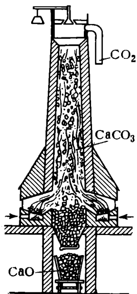
Fig. 180. Limestone roasting shaft kiln
