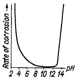
Fig. 207. Relation between the corrosion of zinc and the pH value
