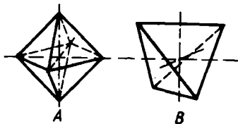
Fig. 198. Octahedron (A) and tetrahedron (B)
