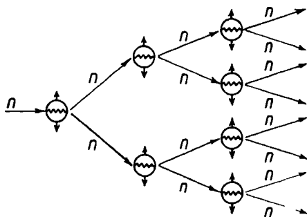
Fig. 233. Diagram of avalanche fission
