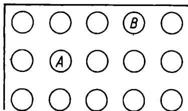
Fig. 99. Origin of an adsorption field
