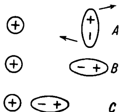
Fig. 84. Orientation of a polar molecule near an ion
