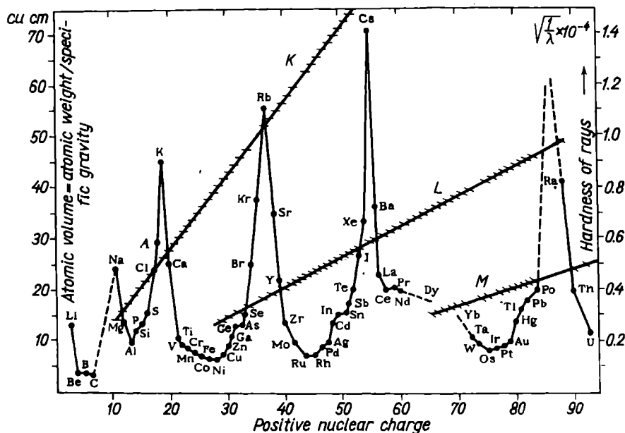
Fig. 208. Periodic and non-periodic properties of the elements
