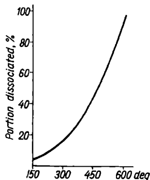
Fig. 120. Equilibrium of thermal dissociation of \text{NO}_2
