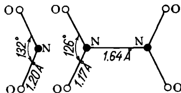
Fig. 119. Spatial structure of \text{NO}_2 and \text{N}_2\text{O}_4
