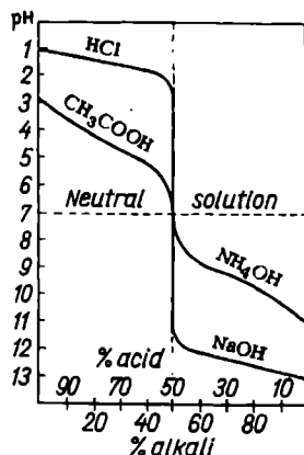
Fig. 89. Change of pH during neutralisation
