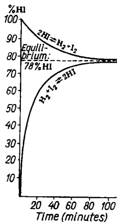
Fig. 71. Two-way approach to equilibrium
