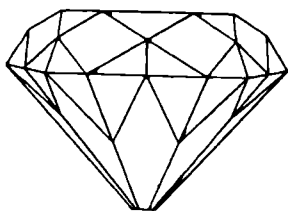
Fig. 130. Diamond facets
