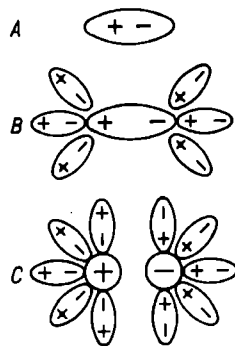
Fig. 86. Transformation of polar structure into ionic structure
