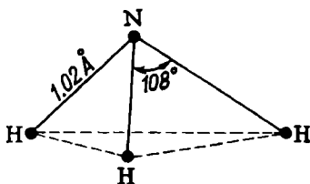
Fig. 113. Structure of the ammonia molecule
