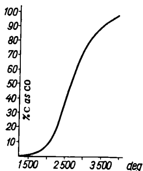
Fig. 133. Equilibrium of the system \text{CO}_2 + \text{C} \rightleftharpoons 2\text{CO}
