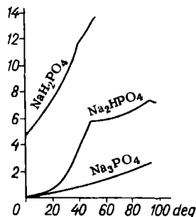
Fig. 127. Solubility of sodium phosphates (moles/litre of \text{H}_2\text{O} )
