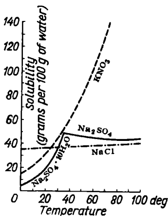
Fig. 80. Solubility curves
