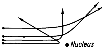
Fig. 26. Deflection of \alpha -particles by a nucleus
