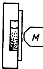
Fig. 21. Diagram of Perrin's experiment
