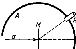
Fig. 25. Diagram of Rutherford's experiment
