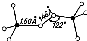
Fig. 107. Structure of the \text{S}_2\text{O}_8^{2-} ion
