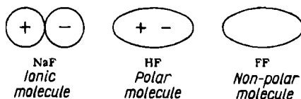
Fig. 42. Different types of molecules
