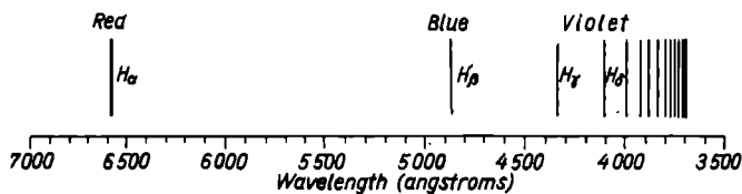
Fig. 62. Visible spectrum of hydrogen (Balmer series)
