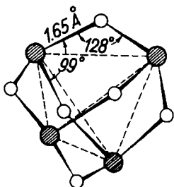
Fig. 125. Spatial structure of \text{P}_4\text{O}_6
