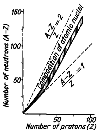
Fig. 222. Compositions of atomic nuclei
