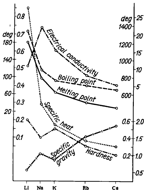
Fig. 185. Properties of the alkali metals
