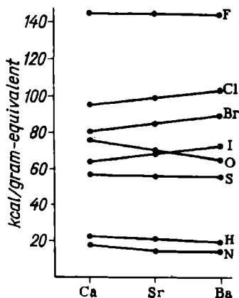
Fig. 178. Heats of formation of Ca, Sr and Ba compounds
