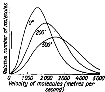
Fig. 59. Velocity-distribution curves of hydrogen molecules
