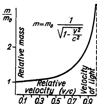
Fig. 223. Mass vs. velocity
