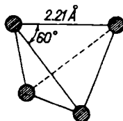
Fig. 124. Structure of \text{P}_4 molecule
