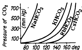
Fig. 190. Dissociation pressure of bicarbonates
