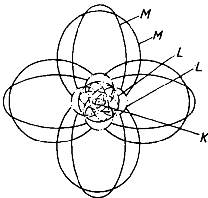
Fig. 69. Model of argon atom
