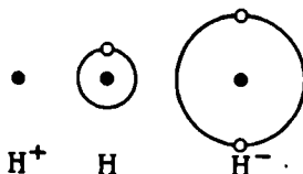
Fig. 60. Atom and ions of hydrogen
