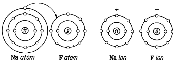
Fig. 40. Diagram of the formation of the NaF molecule according to Kossel
