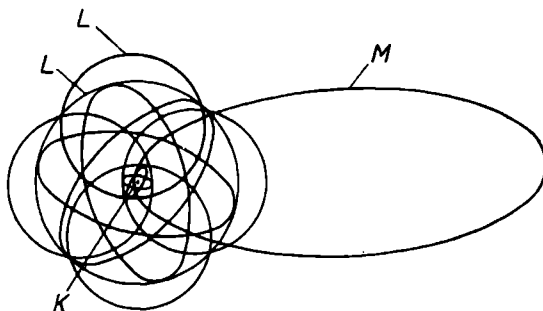
Fig. 68. Model of sodium atom
