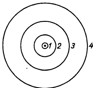
Fig. 63. Possible electronic orbits in the hydrogen atom according to Bohr
