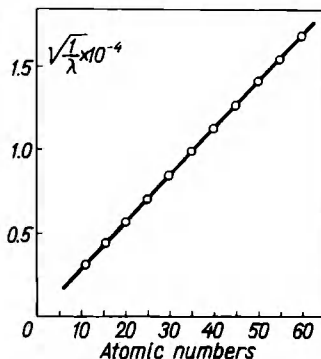
Fig. 34. X-ray wavelengths vs. atomic number
