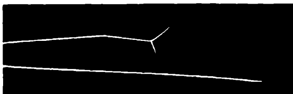
Fig. 29. Tracks of two \alpha -particles
