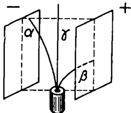
Fig. 22. Splitting up of radioactive radiation in an electric field
