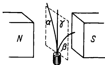
Fig. 23. Splitting up of radioactive radiation in a magnetic field
