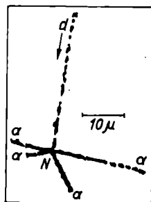
Fig. 229. Transformation of nitrogen into helium
