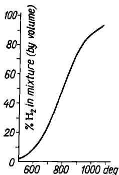
Fig. 136. Equilibrium of methane synthesis
