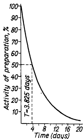
Fig. 215. Decrease in activity of radon
