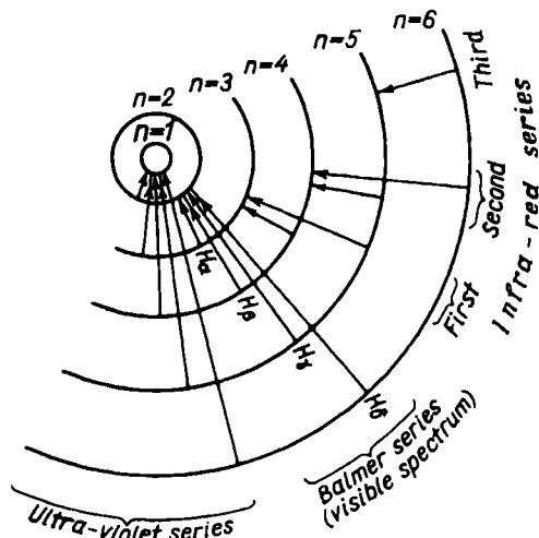
Fig. 64. Diagram of the origin of the hydrogen spectrum
