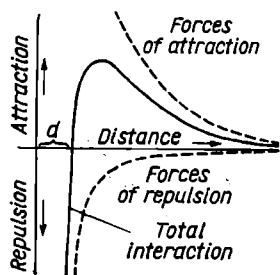
Fig. 50. Forces of attraction and repulsion
