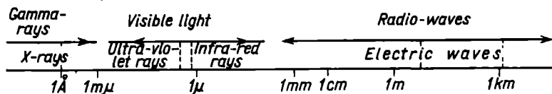
Fig. 30. Electromagnetic spectrum
