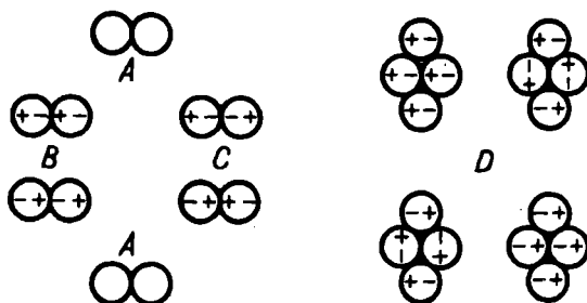
Fig. 49. Diagram of the model treatment of dispersion interaction
