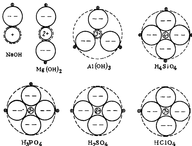
Fig. 87. Type of dissociation depending on charge and radius R
