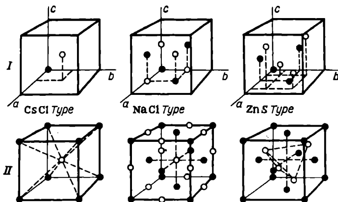
Fig. 171. The most common structures of binary compounds
