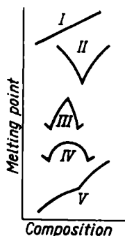
Fig. 159. Curves on freezing-point diagrams
