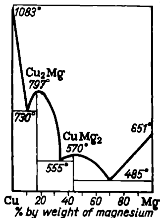
Fig. 162. Freezing-point diagram for the system Cu—Mg
