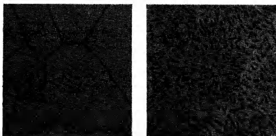
Fig. 161. Microsections of an individual metal and a eutectic
