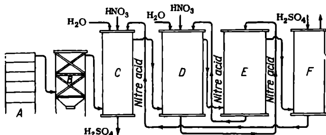
Fig. 105. Diagram of tower plant for manufacture of sulphuric acid
