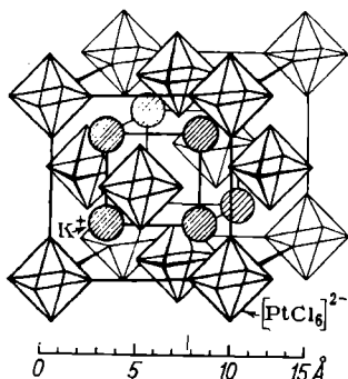
Fig. 199. Crystal structure of K_2[PtCl_6]
