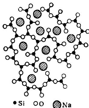
Fig. 146. Arrangement of atoms in sodium silicate glass
