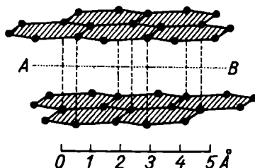
Fig. 131. Arrangement of carbon atoms in graphite
