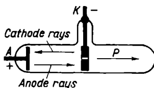
Fig. 216. Diagram of a discharge tube
