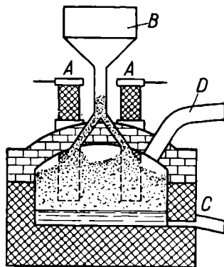
Fig. 123. Diagram of electric furnace for phosphorus production
