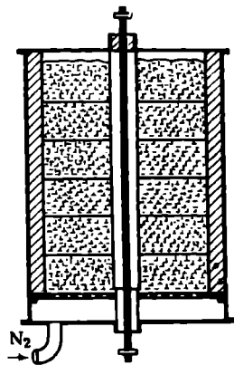
Fig. 112. Diagram of a cyanamide furnace
