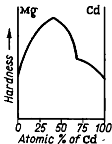
Fig. 155. Hardness of Mg—Cd alloys
