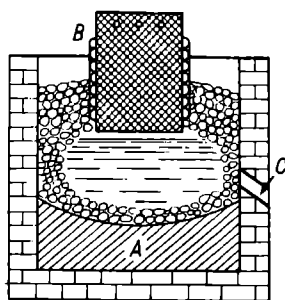
Fig. 139. Calcium carbide furnace
