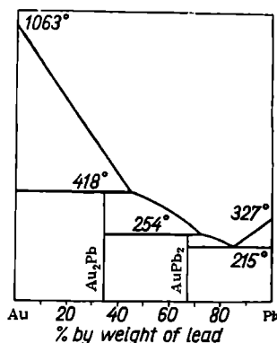
Fig. 163. Freezing-point diagram for the system Au—Pb
