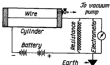
Fig. 212. Diagram of an ionisation counter
