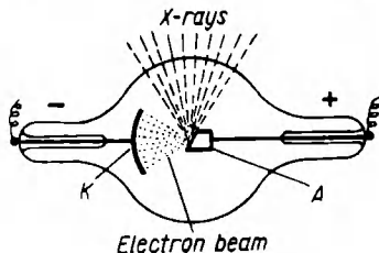
Fig. 32. Diagram of an X-ray tube
