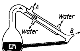
Fig. 182. Mercury vacuum pump
