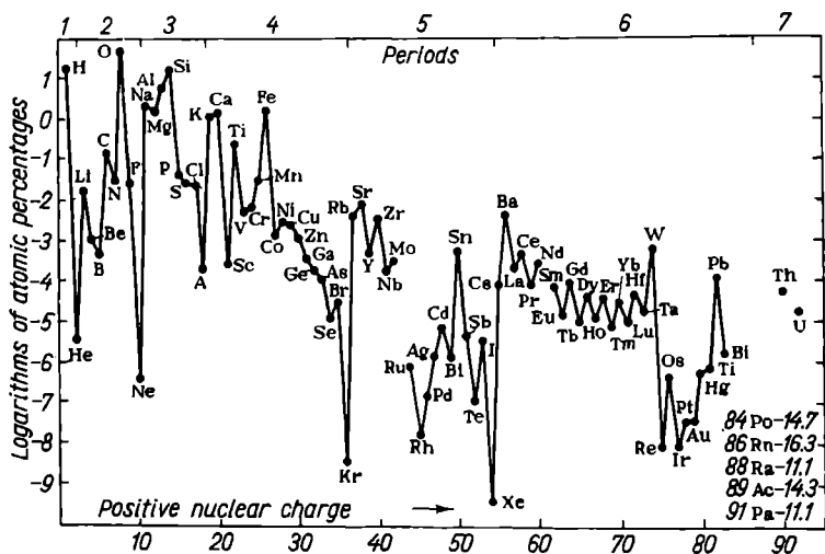
Fig. 209. Relative abundance of the elements in the earth's crust
