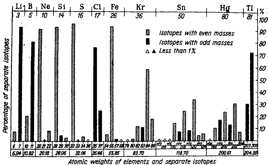
Fig. 219. Isotopic composition of some of the elements
