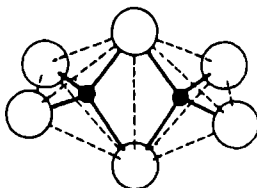
Fig. 152. Structure of an \text{Al}_2\text{X}_6 molecule
