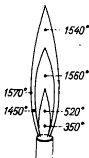
Fig. 137. Flame of a gas burner
