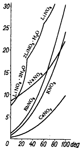
Fig. 189. Solubility of nitrates (moles/litre of \text{H}_2\text{O} )
