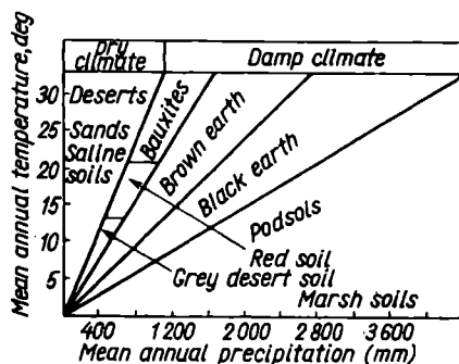
Fig. 144. Diagram of soil-type formation
