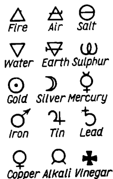
Fig. 4. Alchemical symbols
