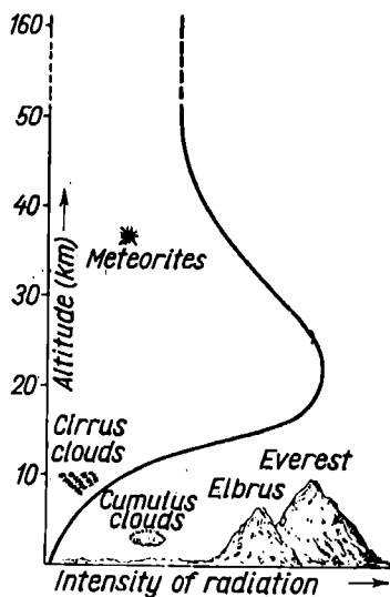
Fig. 220. Intensity of cosmic rays vs. altitude
