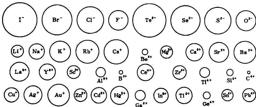
Fig. 177. Relative sizes of ions
