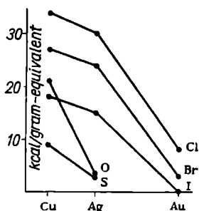
Fig. 197. Heats of formation of Cu, Ag and Au compounds
