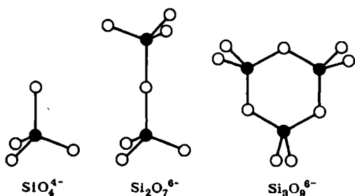
Fig. 142. Simplest silicate anions
