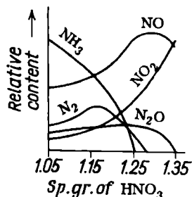
Fig. 122. Products of reduction of \text{HNO}_3 with iron
