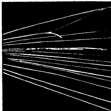
Fig. 226. Collision between an \alpha -particle and a nitrogen nucleus
