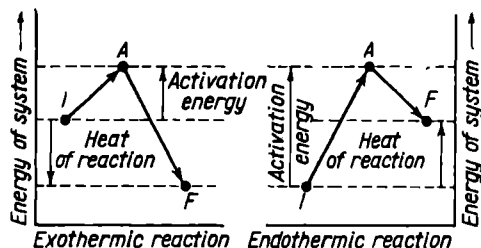
Fig. 70. Diagram of the course of activated reactions
