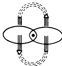
Fig. 39. Interlocking of magnetic fields
