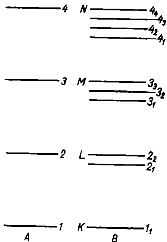
Fig. 67. Diagram of the energy levels for circular and elliptical orbits
