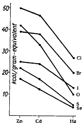
Fig. 183. Heats of formation of Zn, Cd and Hg compounds
