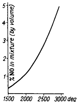
Fig. 117. Equilibrium of synthesis of nitric oxide
