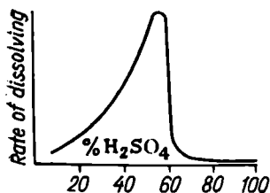
Fig. 205. Reaction between Fe and sulphuric acid
