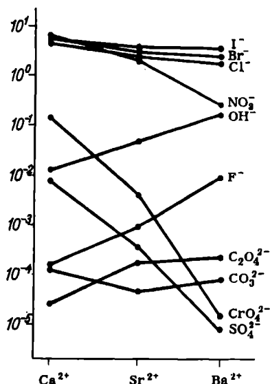
Fig. 179. Solubility of Ca, Sr and Ba salts (moles/litre of \text{H}_2\text{O} )
