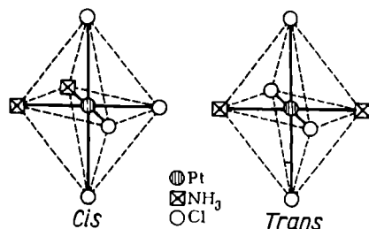
Fig. 201. Diagram of cis-trans isomerism
