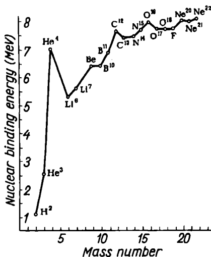
Fig. 224. Binding energies of the lighter atoms
