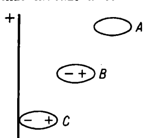
Fig. 45. Polarisation of a non-polar molecule
