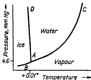
Fig. 78. Phase diagram of water
