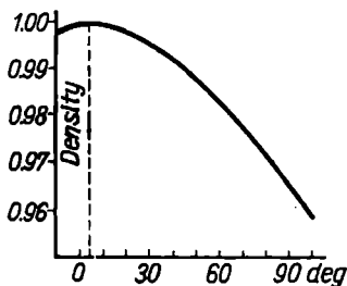
Fig. 76. Water density vs. temperature
