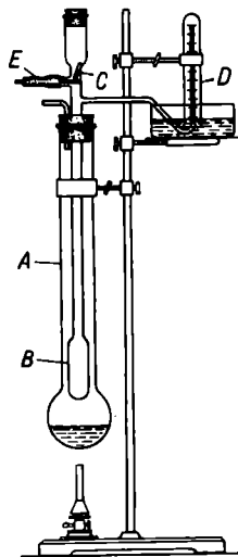
Fig. 8. Apparatus for determining molecular weight
