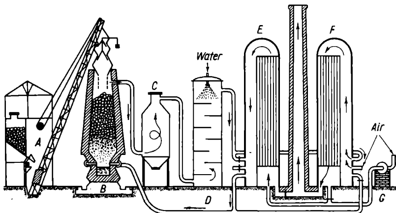
Fig. 203. Blast-furnace plant of a steel works
