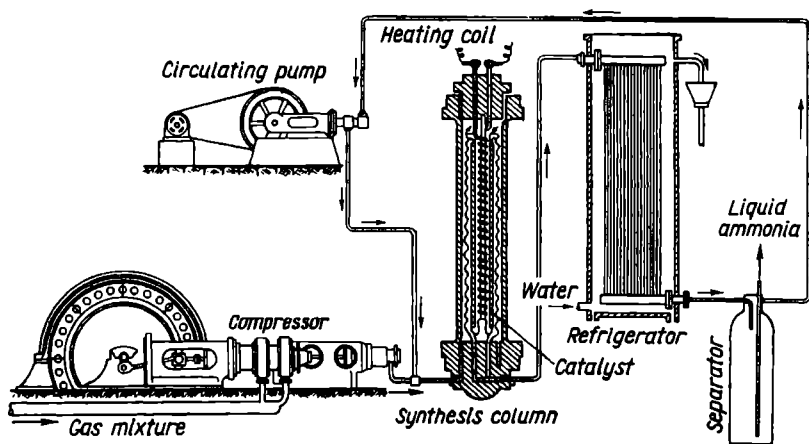
Fig. 111. Diagram of ammonia synthesis plant
