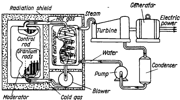
Fig. 237. Key diagram of installation for utilising nuclear energy
