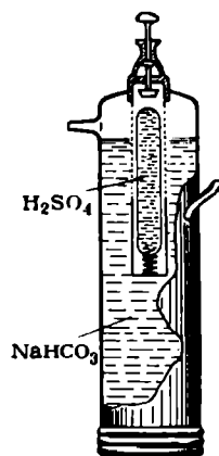
Fig. 132. A fire extinguisher (cut-away view)
