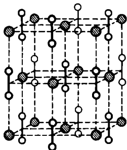
Fig. 138. Structure of a \text{CaC}_2 crystal
