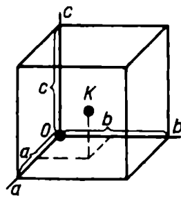
Fig. 170. An example of a unit cell
