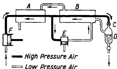
Fig. 10. Diagram of a liquid air plant
