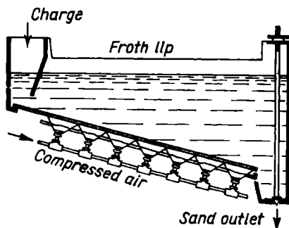
Fig. 195. Schematic representation of the flotation process
