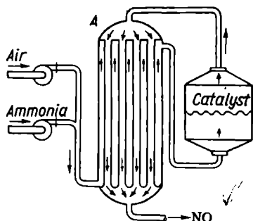
Fig. 121. Diagram of a plant for the catalytic oxidation of ammonia
