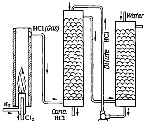
Fig. 97. HCl synthesis plant
