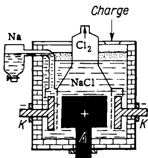
Fig. 184. An electrolytic cell for the preparation of sodium
