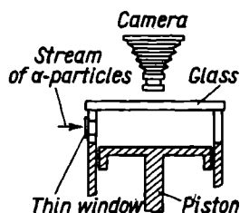
Fig. 27. Diagram of a cloud chamber
