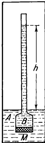
Fig. 82. Determining osmotic pressure
