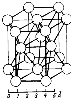
Fig. 175. Lattice of metallic magnesium
